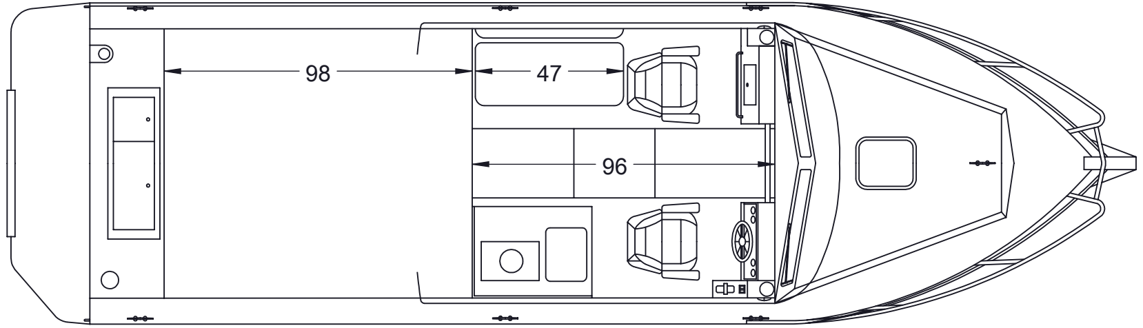
260 CUDDY KING 96" CABIN FLOOR PLAN 96-6
