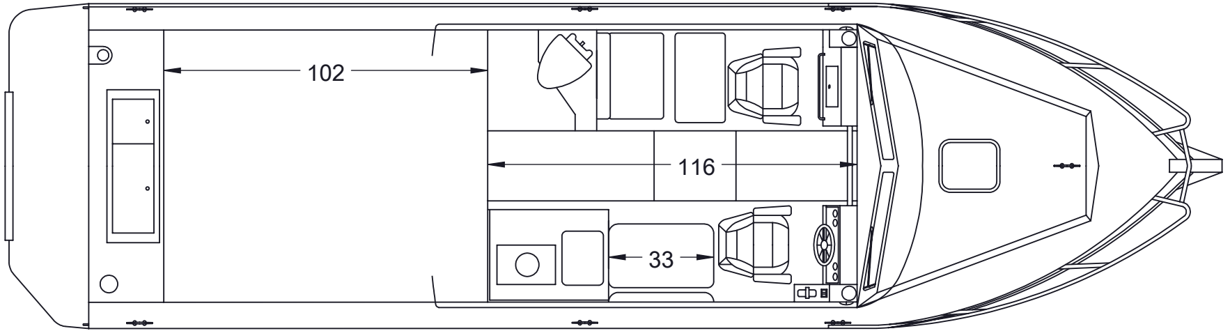
280 CUDDY KING 116" CABIN FLOOR PLAN 116-8
